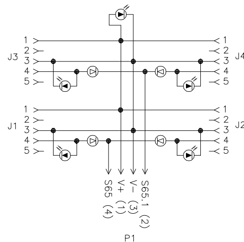
WIRING DIAGRAM
